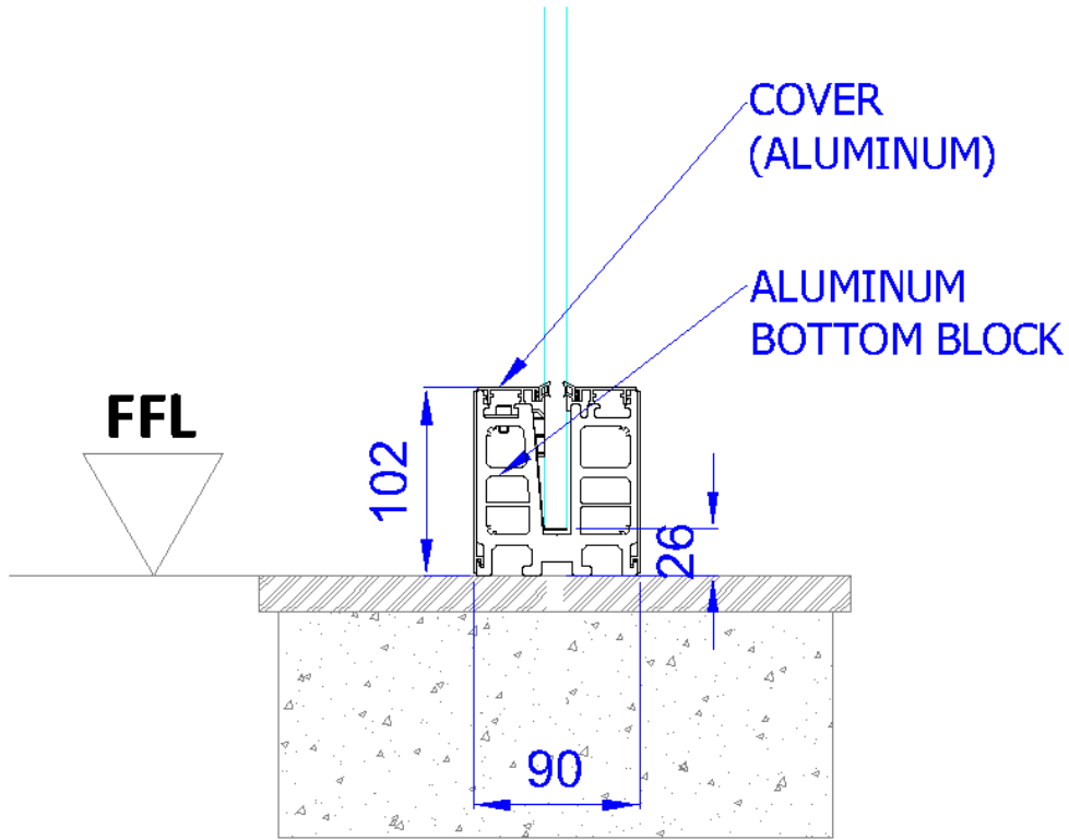
SIDE VIEW
